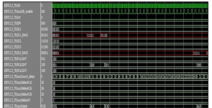
Fig. 19. The timing diagram for the real-time density-based traffic system with road blockage signal.
